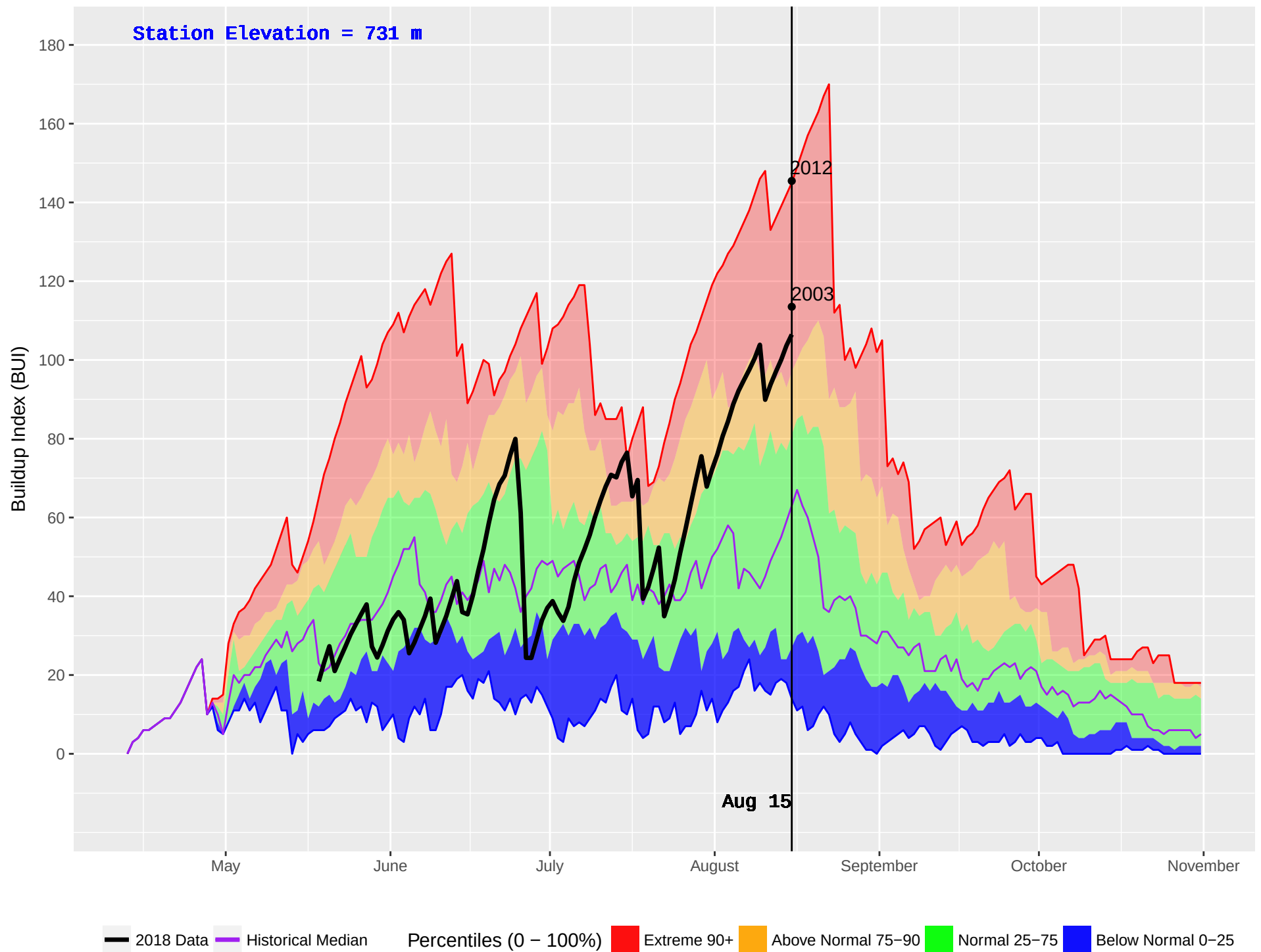
FIRESIDE (440) : Historical (1996–2016) and Current (2018) Daily Buildup Index (BUI)
