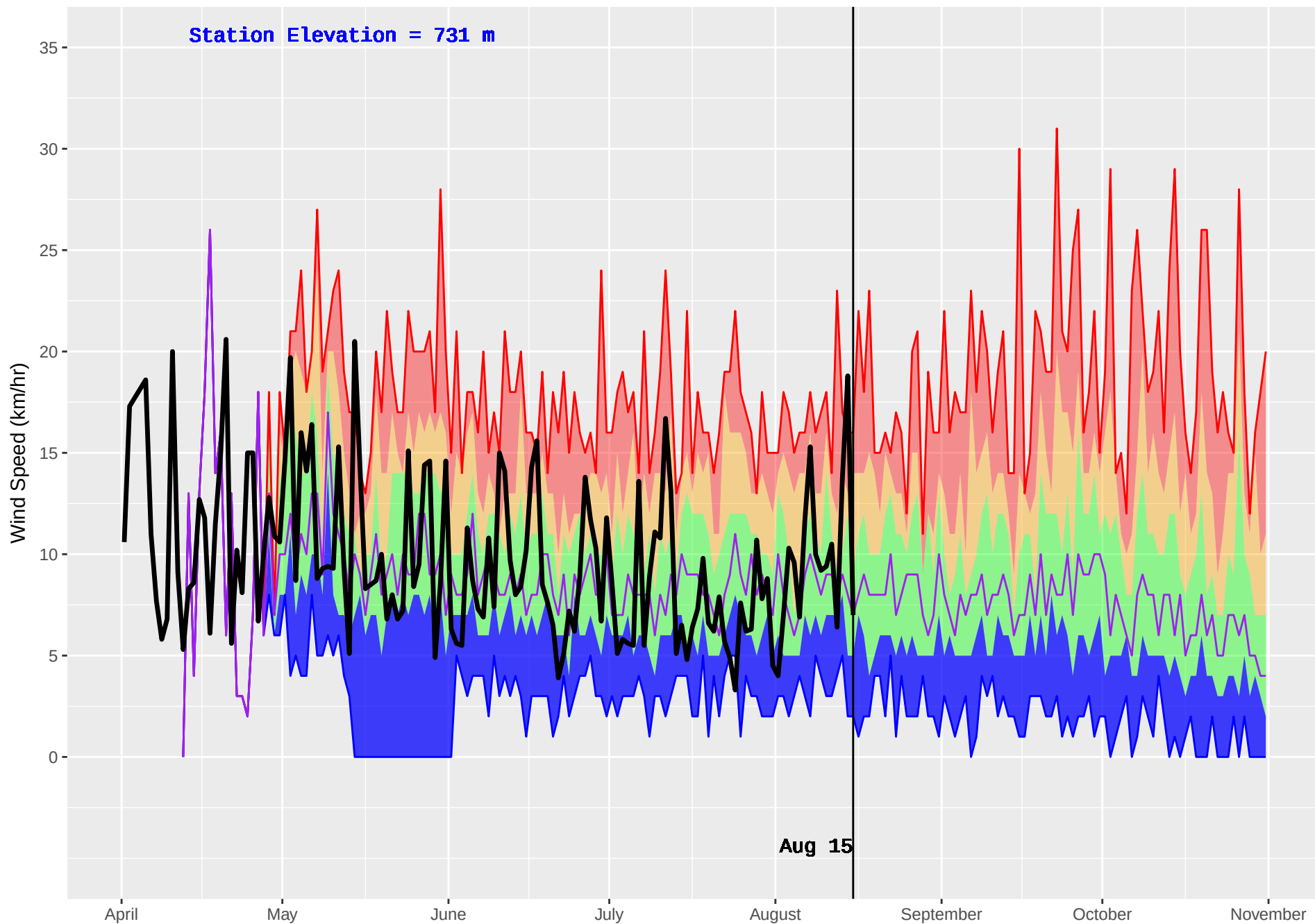
FIRESIDE (440) : Historical (1996–2016) and Current (2018) Daily Wind Speed
